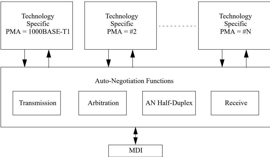
Figure 98–2—High-level model
