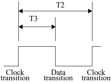
Figure 98–9—DME page transition timing
