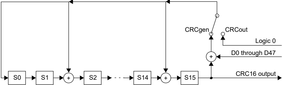
Figure 98-6—CRC16
