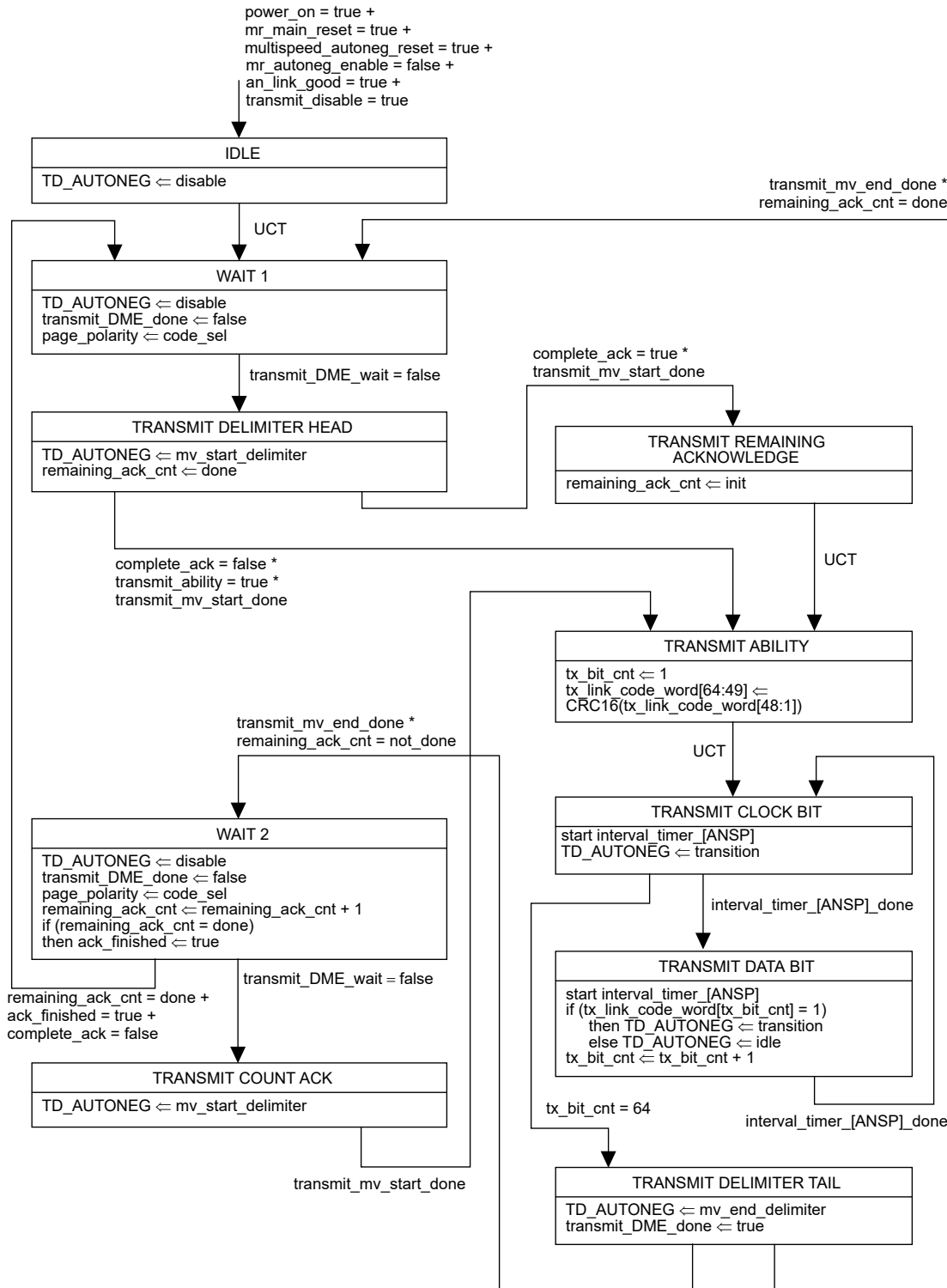
Figure 98–16—Transmit state diagram
