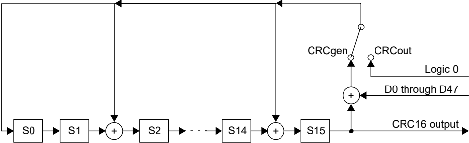
Figure 98-5—CRC16
