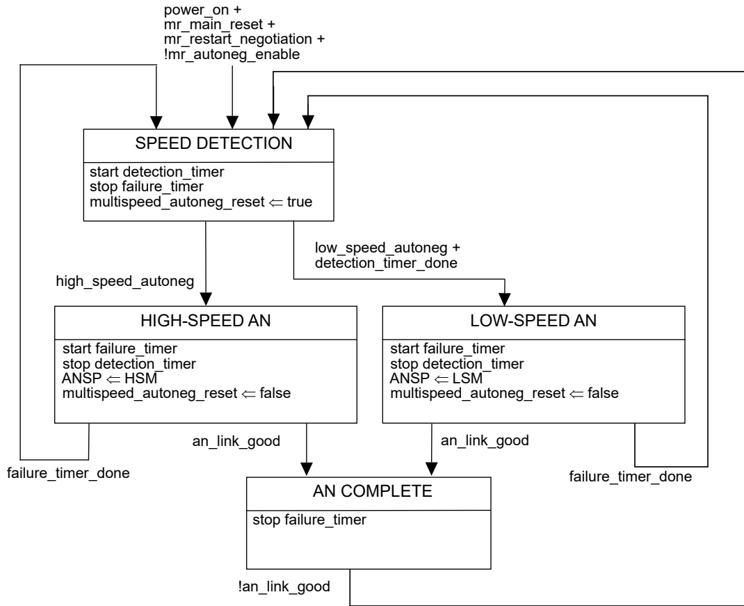
Figure 98–21—Auto-Negotiation—high-speed mode and low-speed mode selection
