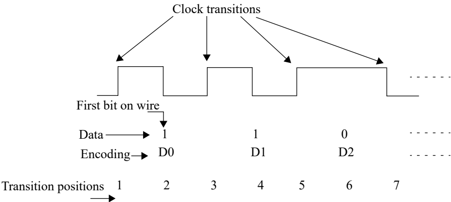
Figure 98-7—Data bit encoding within DME pages
