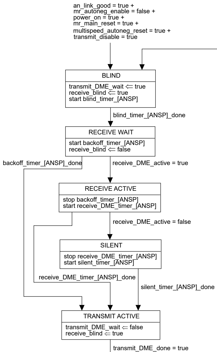
Figure 98–18—Half-duplex state diagram
