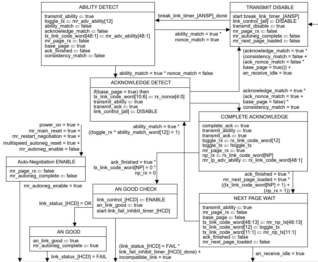
Figure 98–13—Arbitration state diagram
