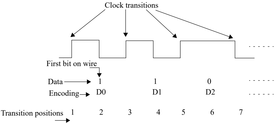
Figure 98-8—Data bit encoding within DME pages
