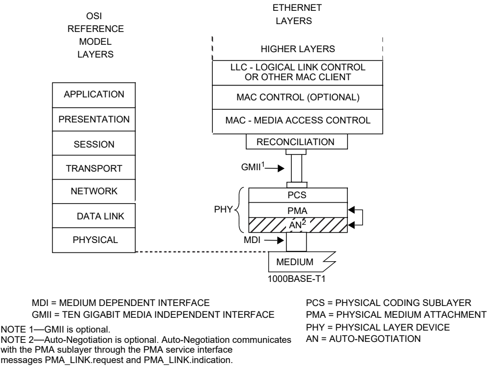
Figure 98–3—Location of Auto-Negotiation function within the ISO/IEC OSI reference model
