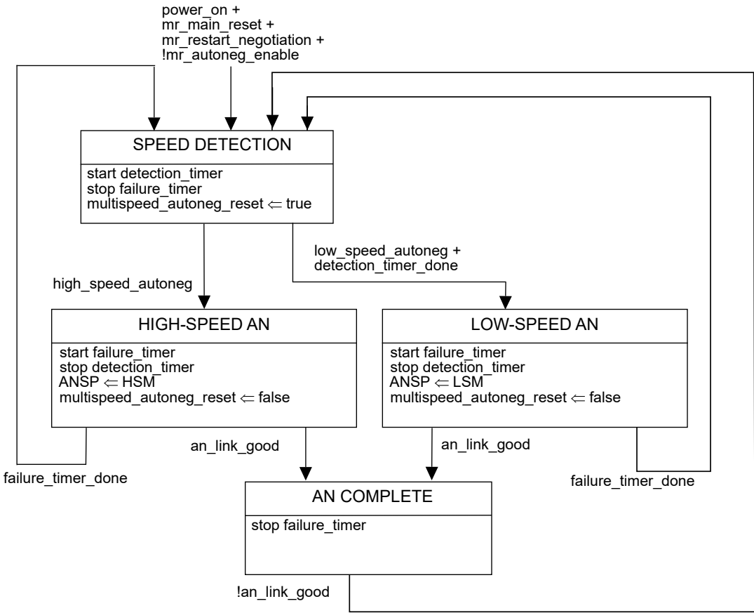
Figure 98–22—Auto-Negotiation—high-speed mode and low-speed mode selection
