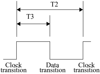
Figure 98–10—DME page transition timing
