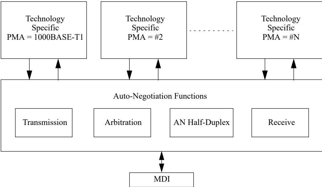
Figure 98–1—High-level model
