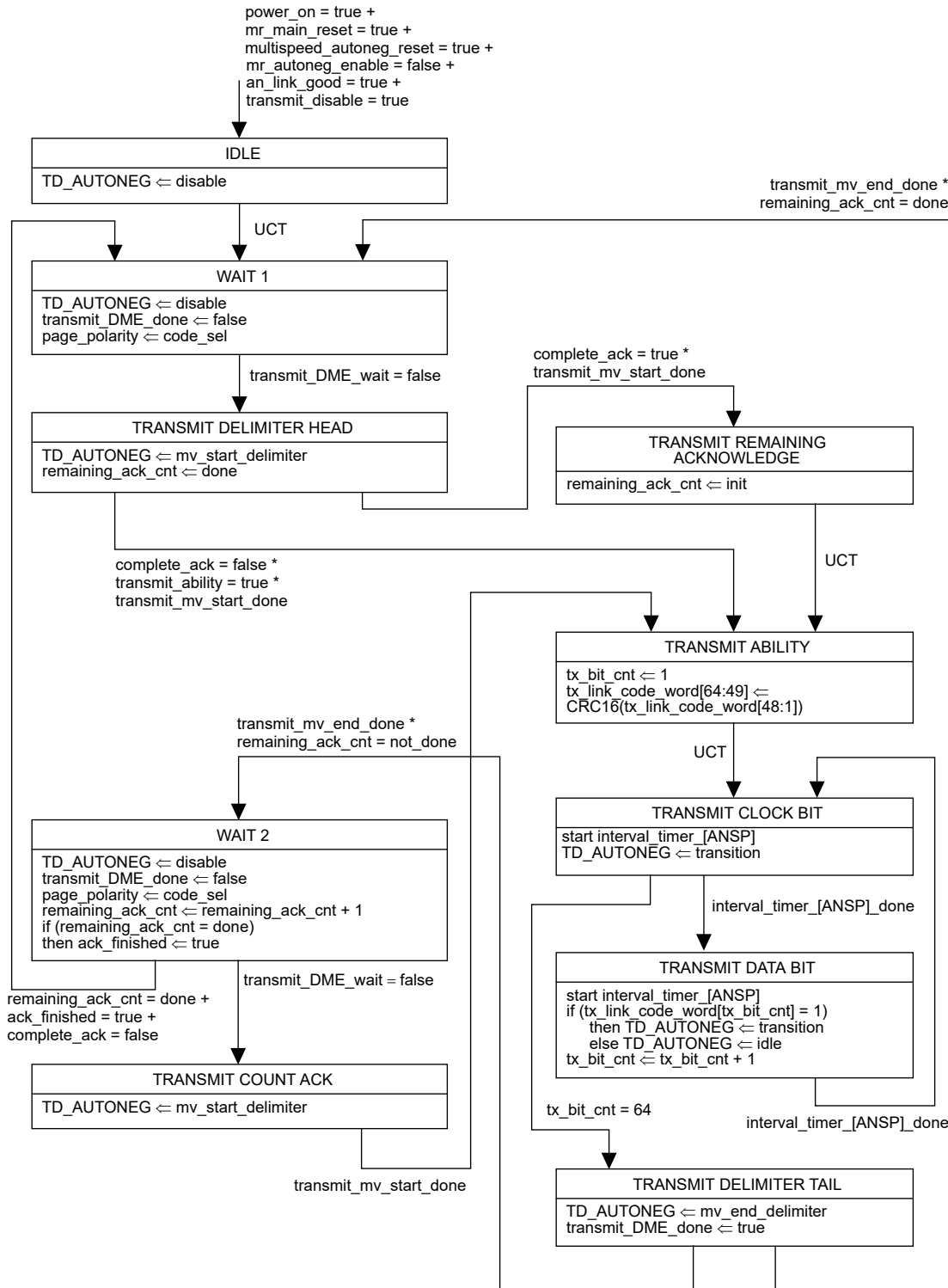
Figure 98–14—Transmit state diagram
