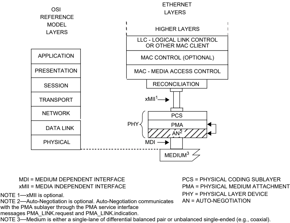
Figure 98-4—Location of Auto-Negotiation function within the ISO/IEC OSI reference model
