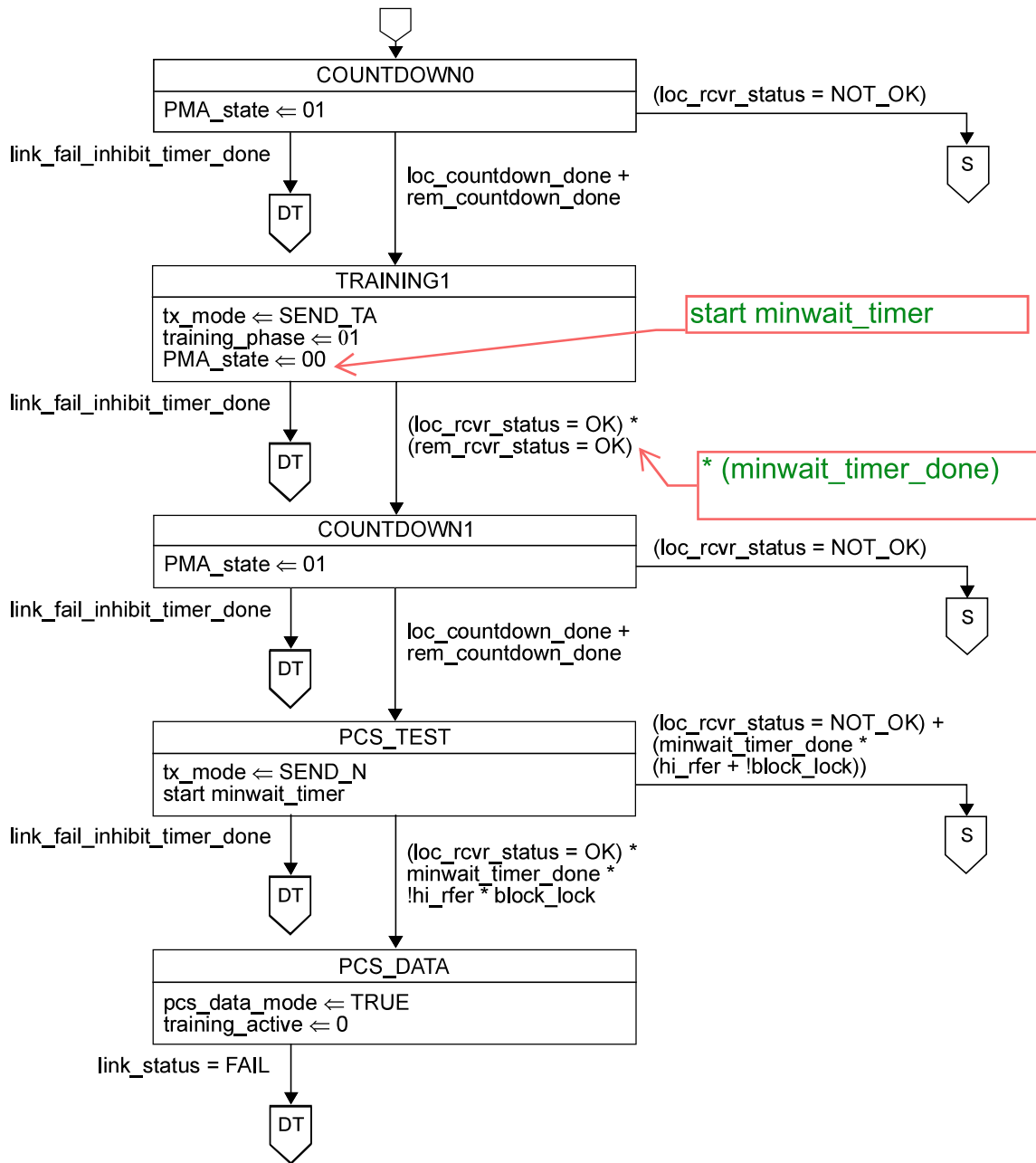
Figure 202-27—PHY Control state diagram, part b
