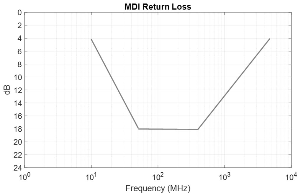
Figure 200-2—MDI return loss calculated using Equation (200-1)
