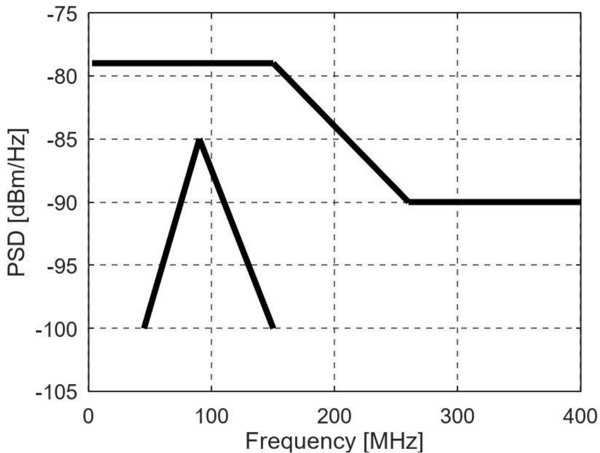
Figure 200.9-1—PSD masks for low speed as specified by Equations (200.8-1) and (200.8-2)
