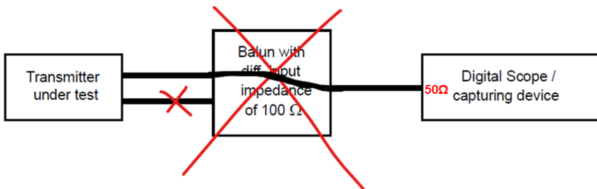
Figure 200.9.1.1—3—Transmitter test fixture 3 for MDI jitter measurement
