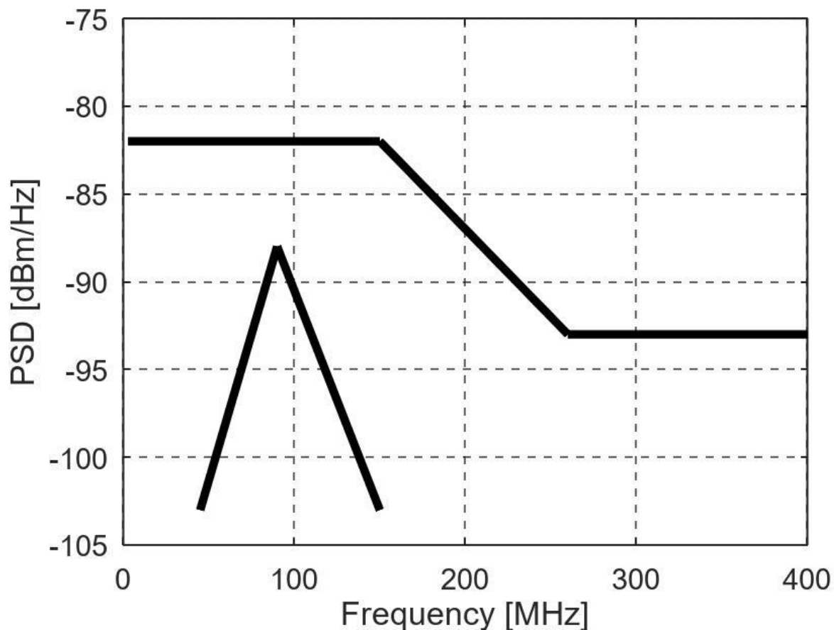
Figure 200.9-1—PSD masks for low speed as specified by Equations (200.9-1) and (200.9-2)
