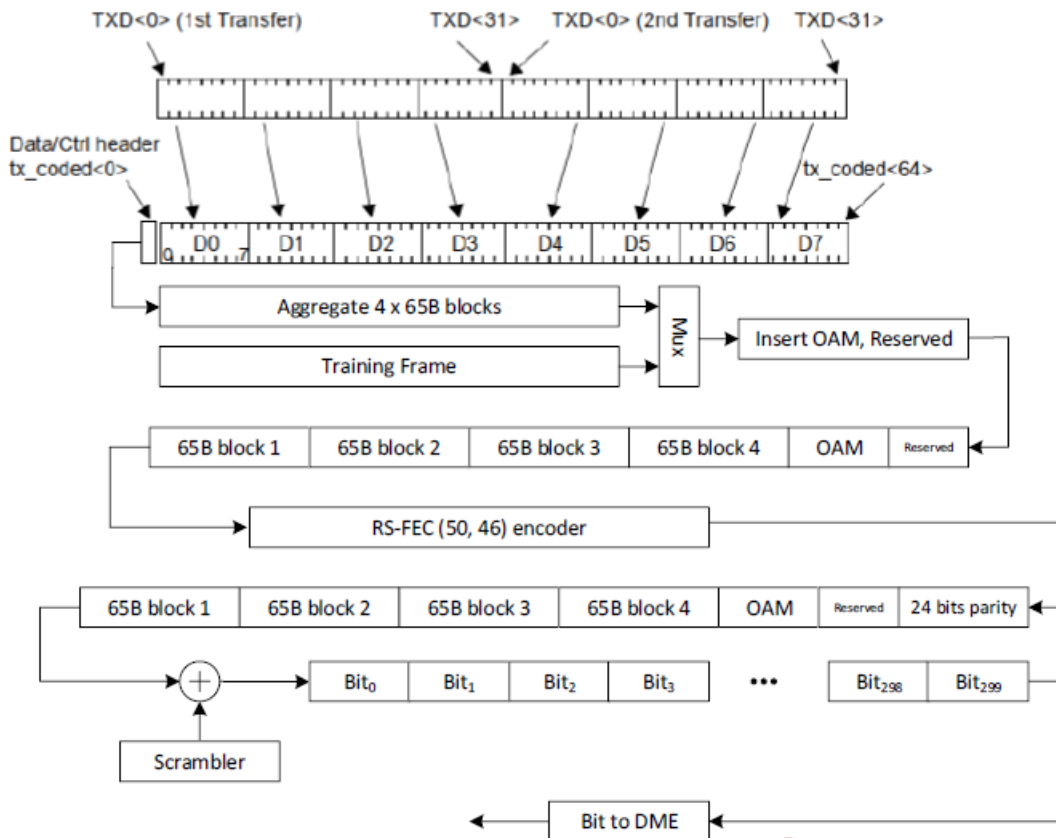
Figure 200–5 – PCS Transmit bit ordering for data mode and training mode
