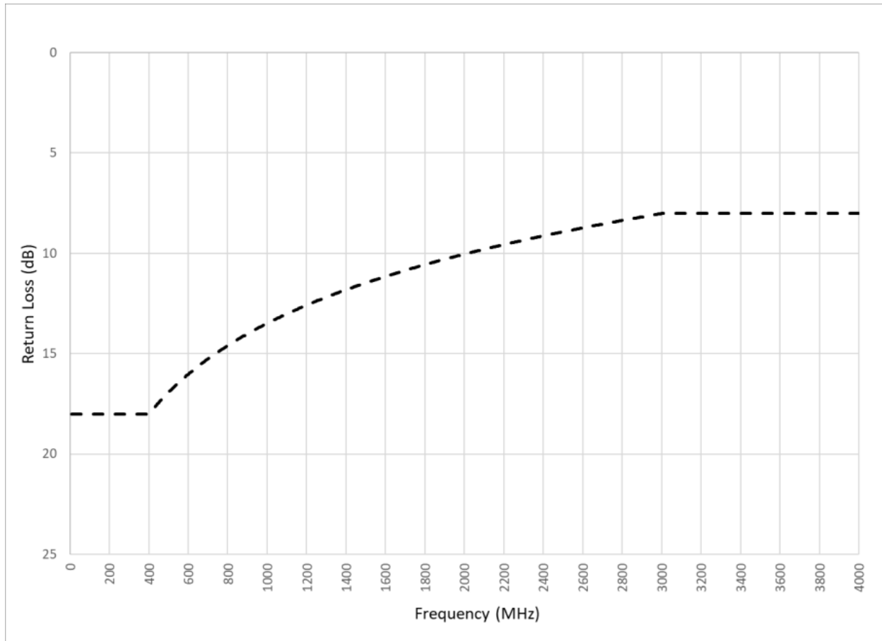
Figure 200-11.1.3 - Return loss limit
