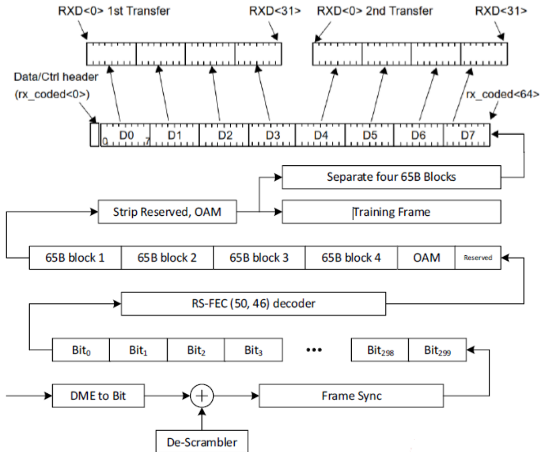
Figure 200.5.2 Demapping of data mode and training frame
