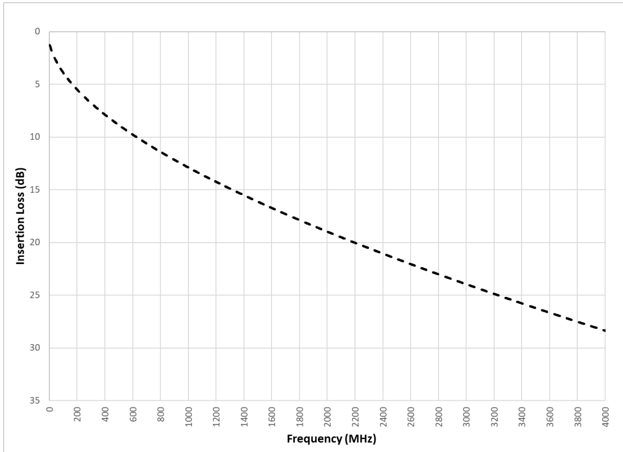
Figure 200.11.1.1 Insertion loss limit for balanced pair and coaxial cables
