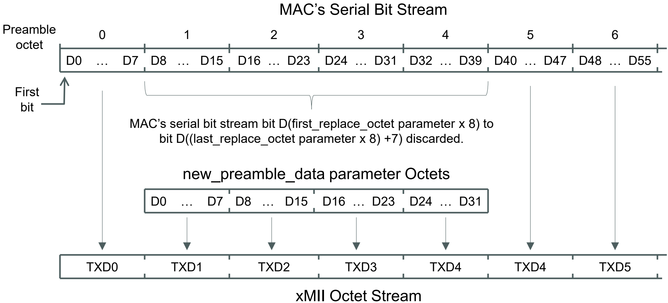
Figure XXX–3 Servicing an EMS_PA.request with first_replace_octet parameter set to 1 and last_replace_octet parameter set to 4
