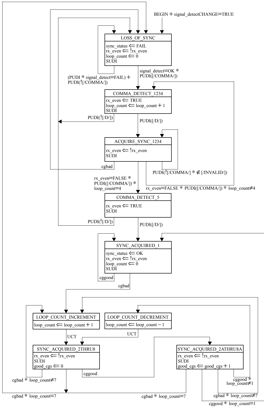
Figure 57-10—Receive byte alignment state diagram
