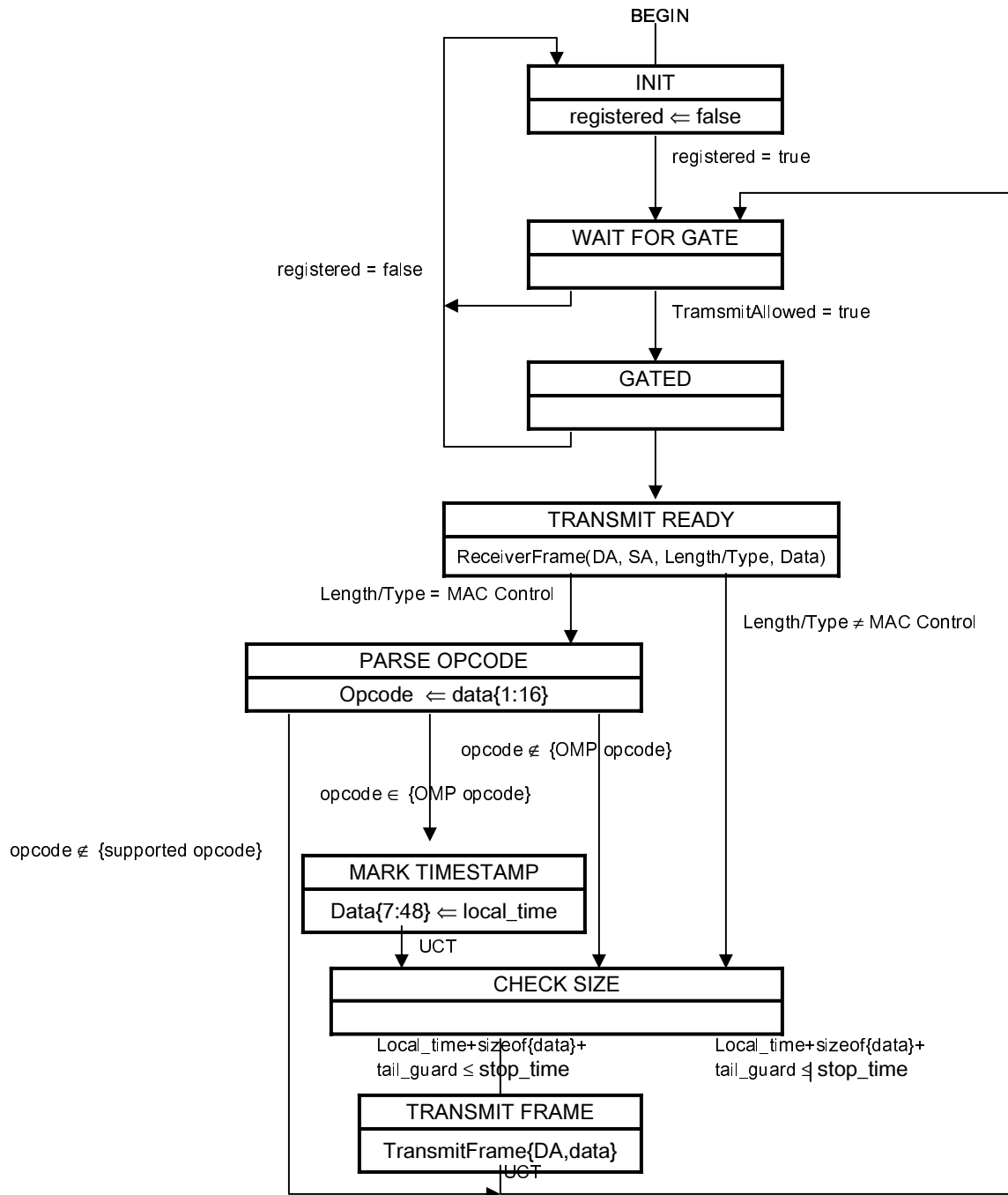
Figure 64-12 ONU Control Multiplexer State Diagram
