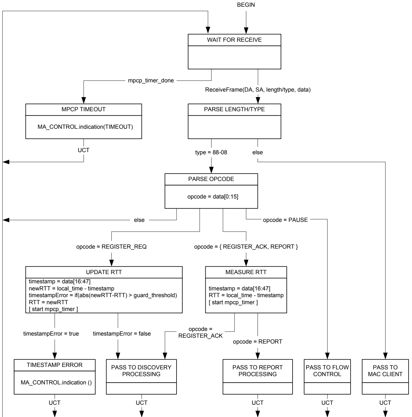
OLT Parser state diagram
