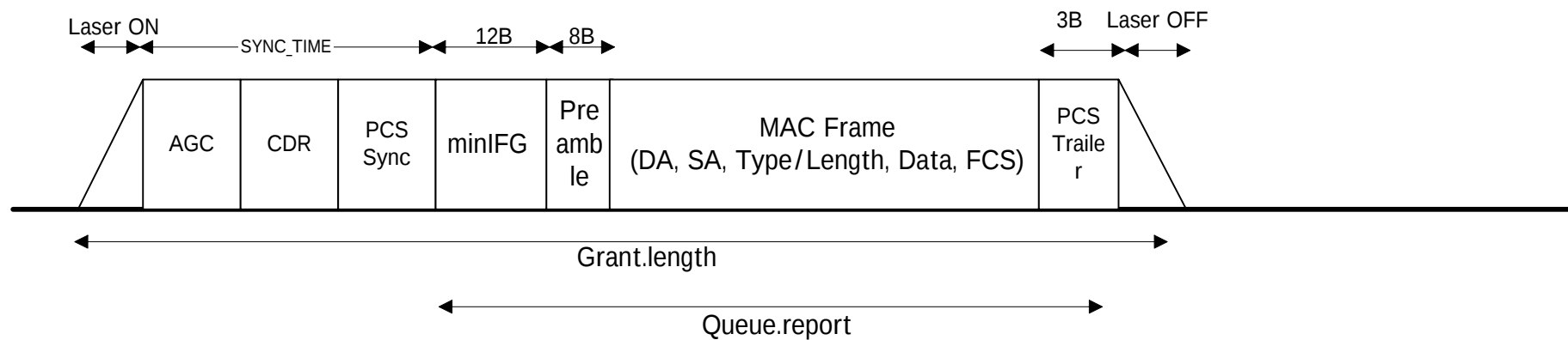
Fig1: One frame transmission from ONU
