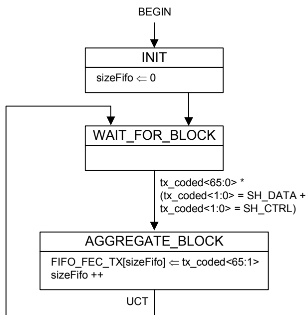
Figure 101–2—FEC encoder Encode and Data Detector , input process state diagram
