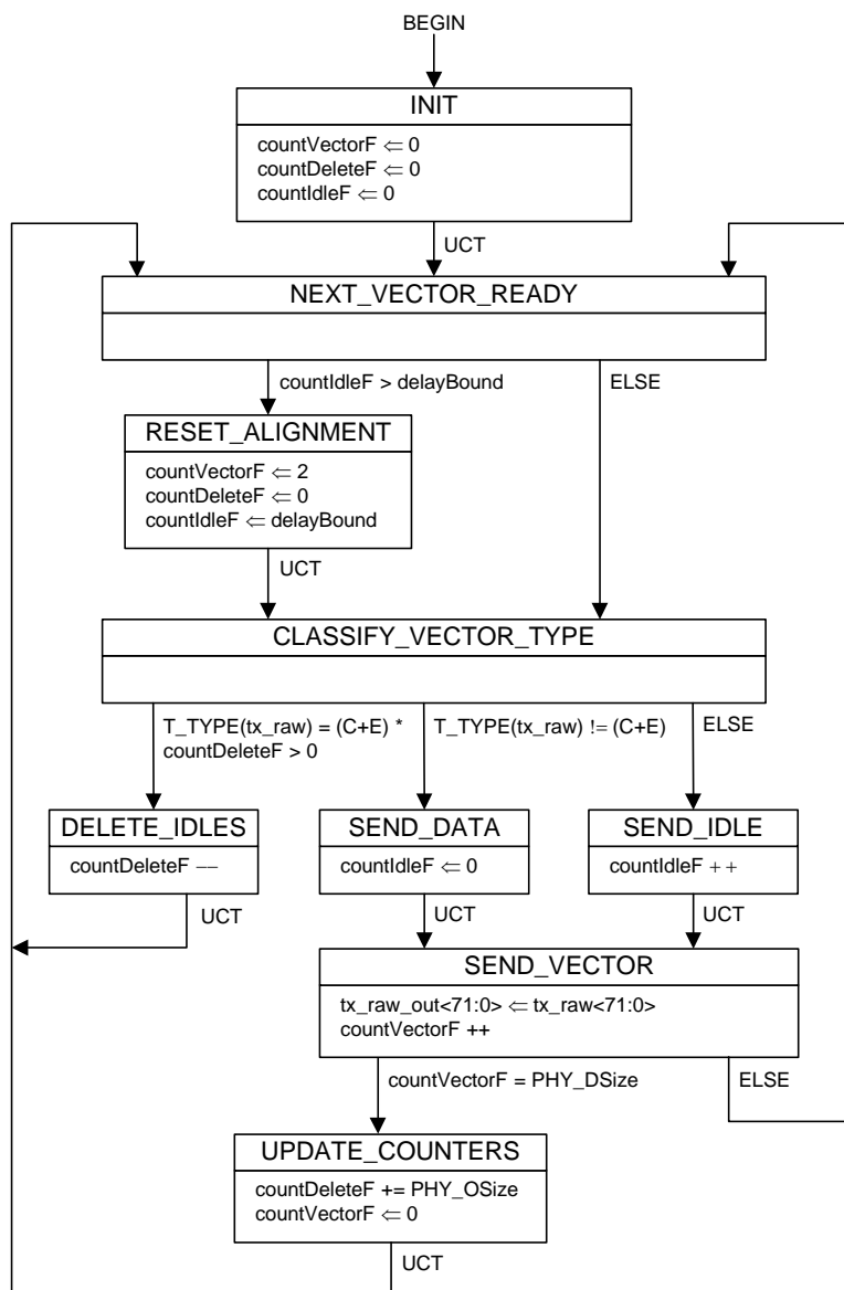
Figure 101–4—CNU Idle control character deletion process (FEC overhead compensation sub-process)
