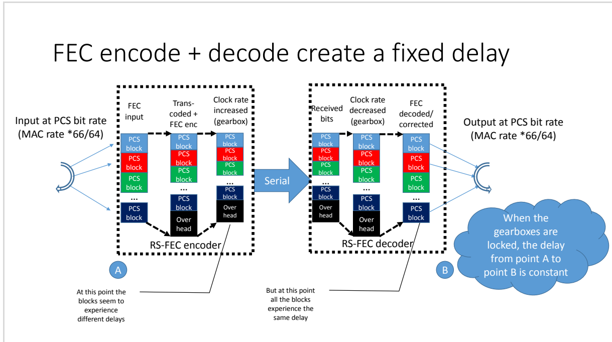
Figure 1: Synchronous FEC encoding and decoding
