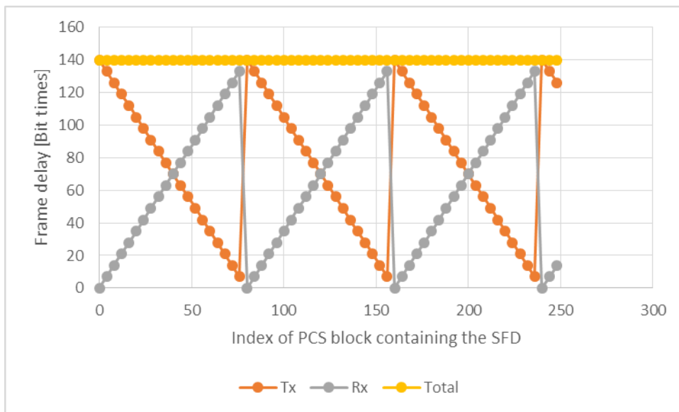
Figure 2: Frame delay due to transcoding in RS(528,514)
