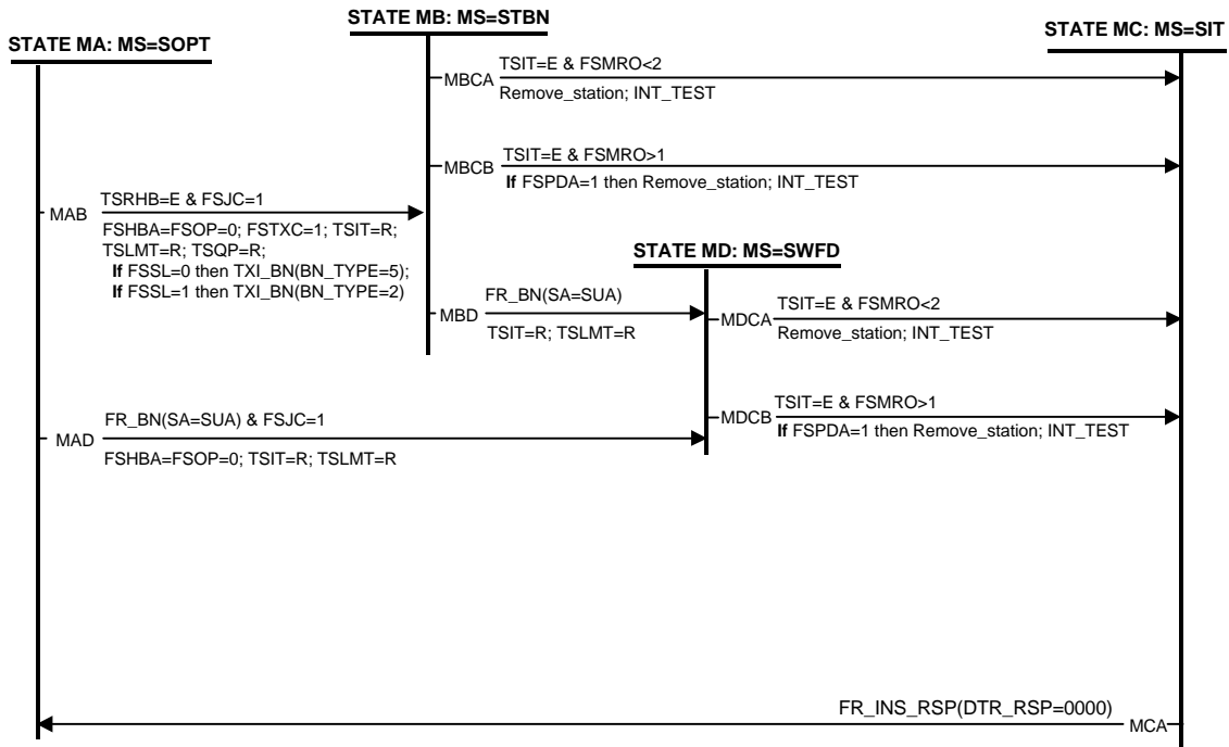
Figure L-3 - MONITOR FSM
