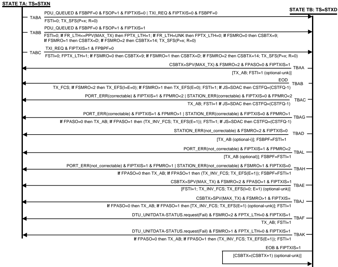
Figure L-2 - TRANSMIT FSM
